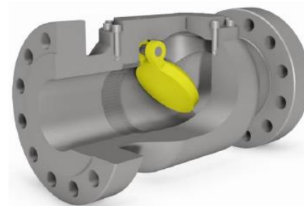
SWING AND DUAL PLATE CHECK VALVE
